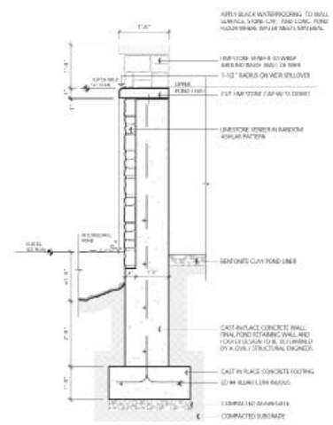
UPPER AND LOWER POND RETAINING WALL / OVERFLOW WIER NTS
